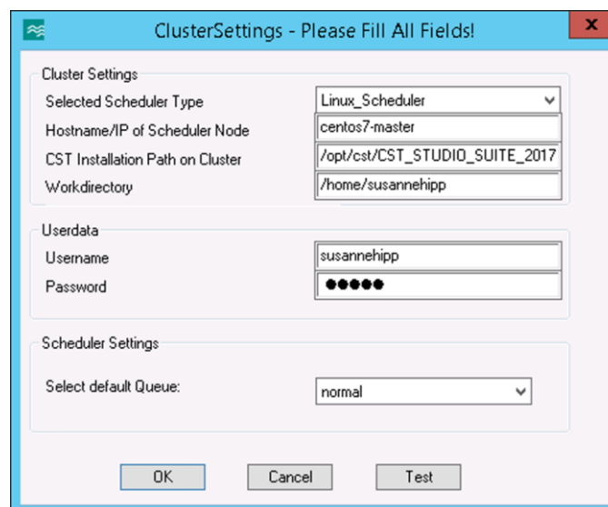
Figure 4: Configuration Wizard for Linux.
