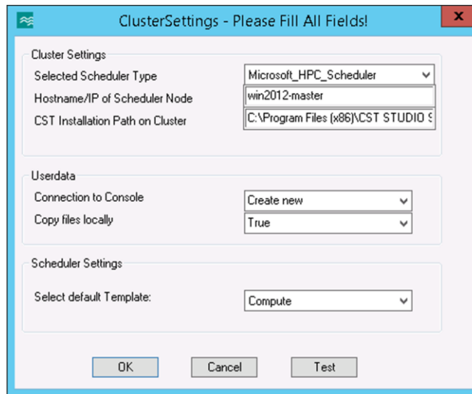
Figure 5: Configuration Wizard for Microsoft HPC Scheduler.
