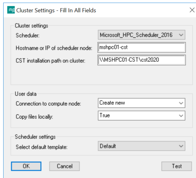
Figure 4: Configuration Wizard for Windows schedulers.
