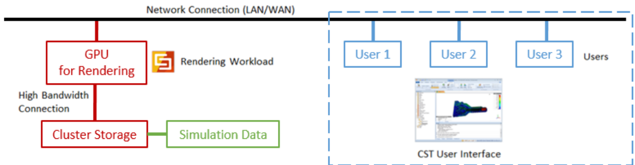
Figure 9: Remote access to simulation data using GPU accelerated rendering and remote access protocol. The picture shows the principle setup and the involved system components.
