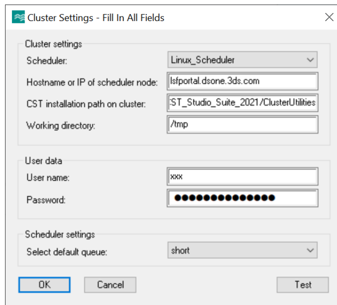
Figure 5: Configuration Wizard for Linux schedulers.
